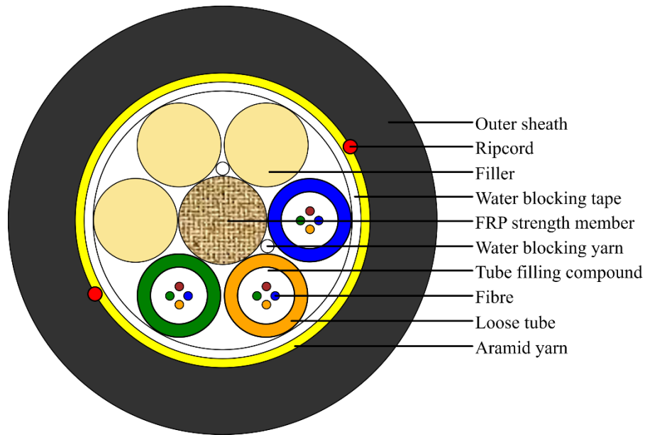
ADSS-SS-100M-12B1.3
